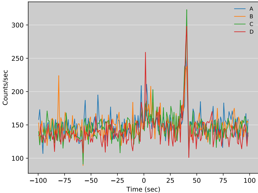
GRB Lightcurve, T0 = 350430731.0
