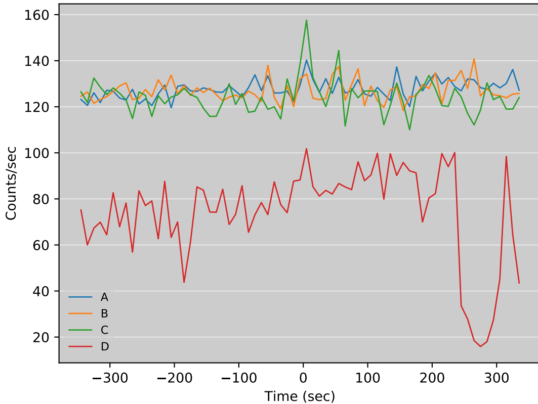
GRB Lightcurve, T0 = 349351208.0
