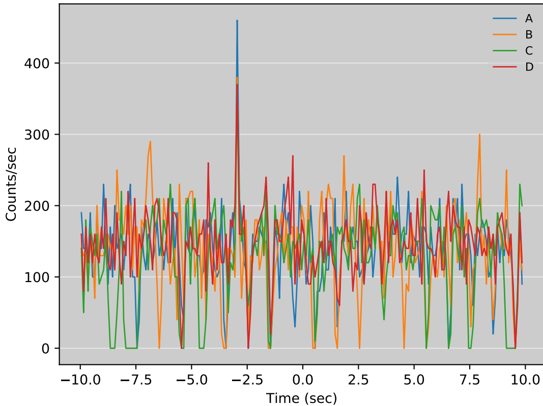
GRB Lightcurve, T0 = 349190631.4
