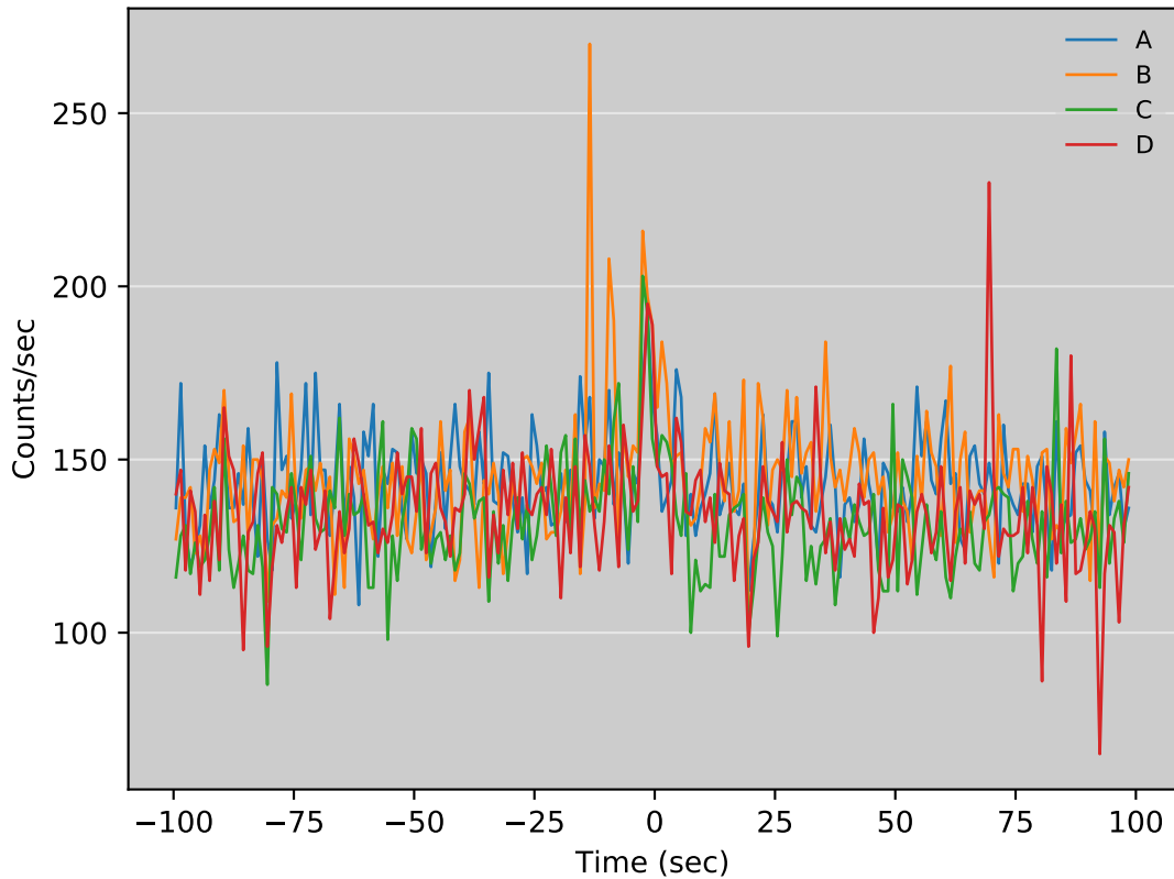
GRB Lightcurve, T0 = 349082353.35
