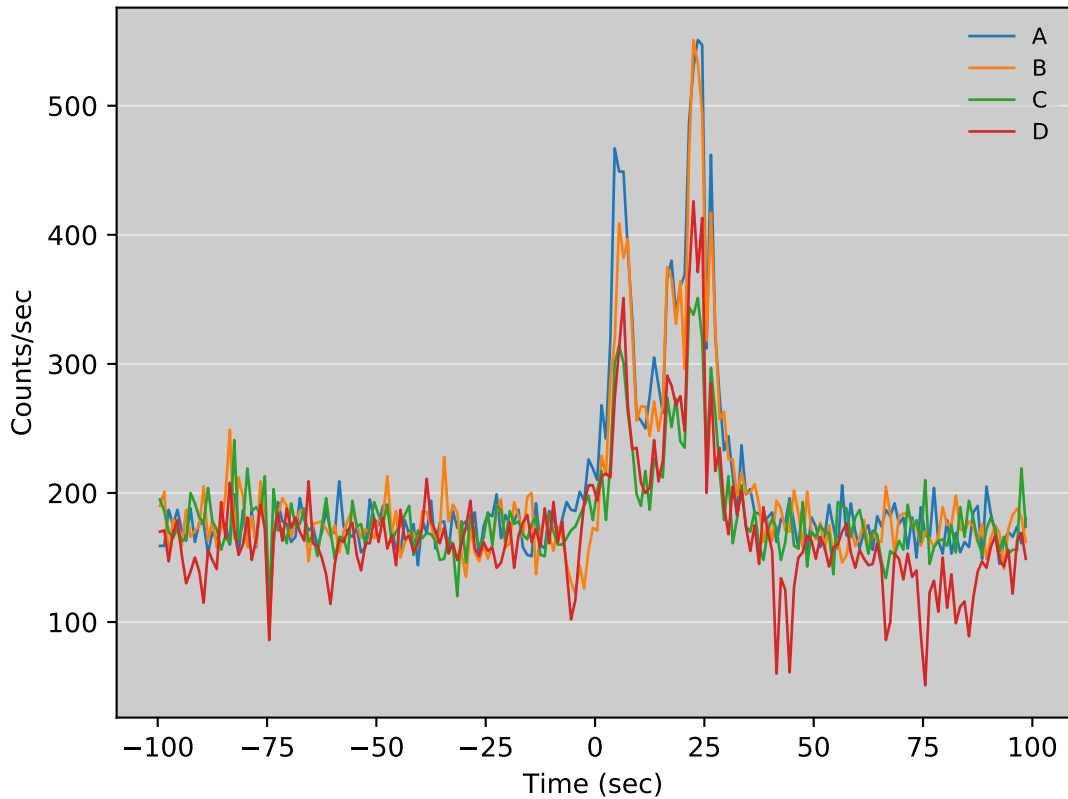
GRB Lightcurve, T0 = 345856048.0
