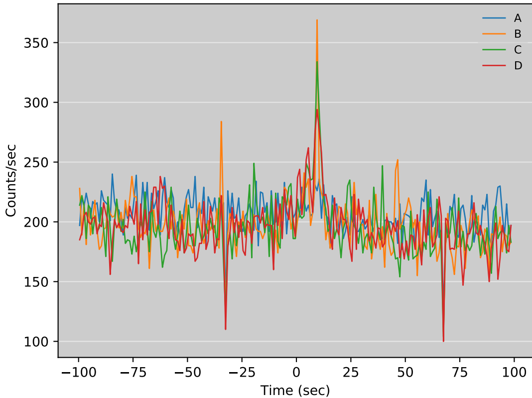
GRB Lightcurve, T0 = 345103406.0
